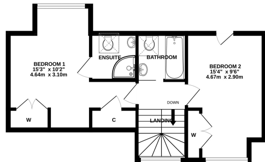
1ST FLOOR 445 sq.ft. (41.3 sq.m.) approx.
