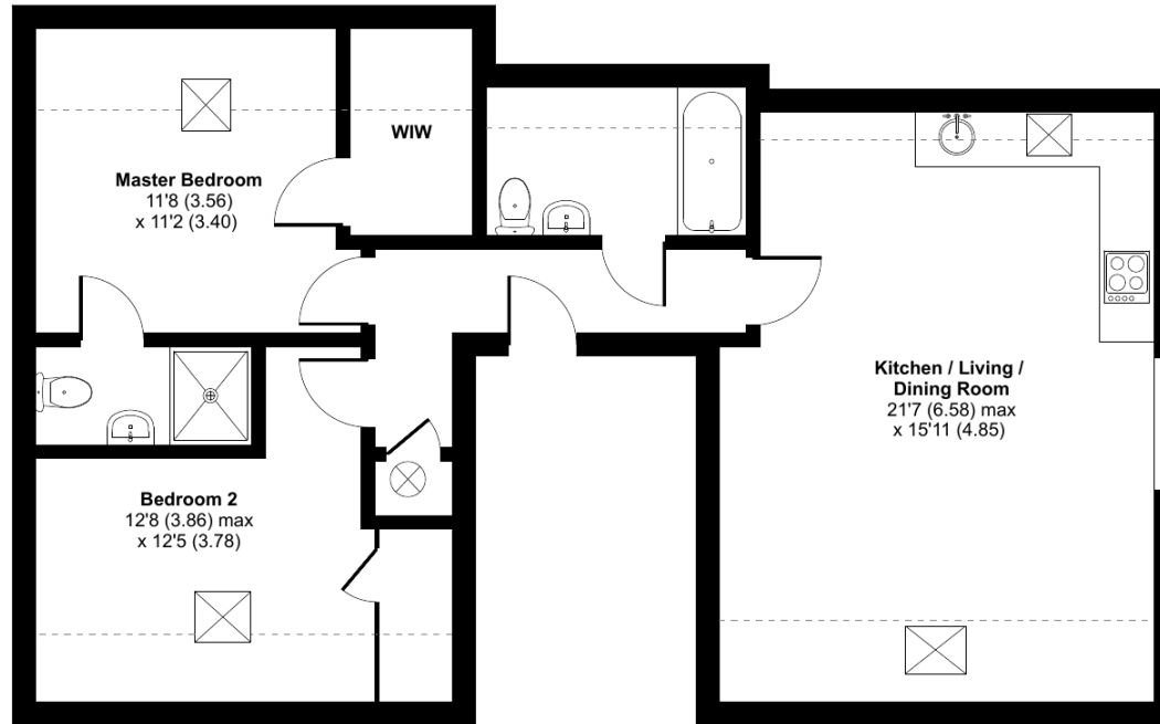
FOURTH FLOOR
