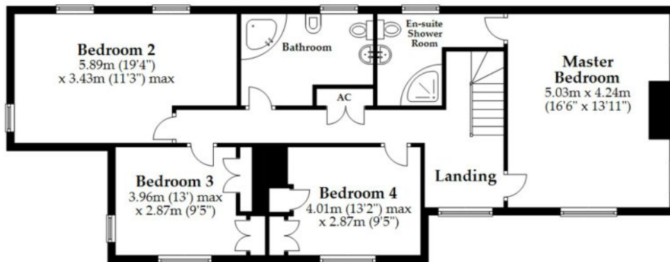
First Floor Approx. 94.4 sq. metres (1016.4 sq. feet)
