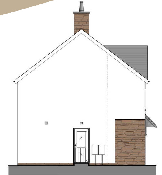
SIDE 1 ELEVATION
