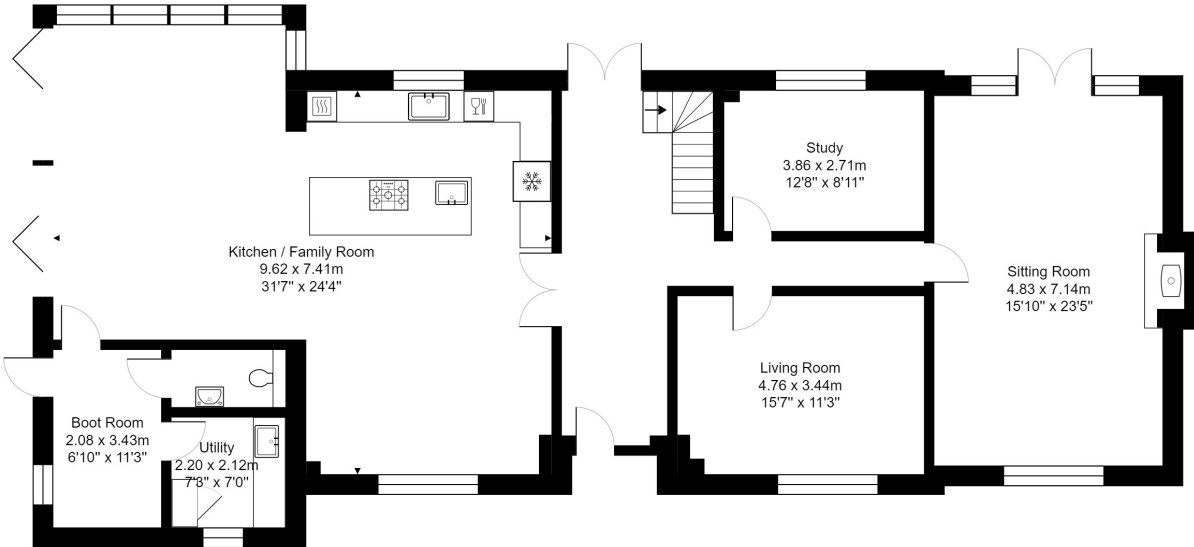
Ground Floor Area: 166.5 m 2 ... 1792 ft 2
