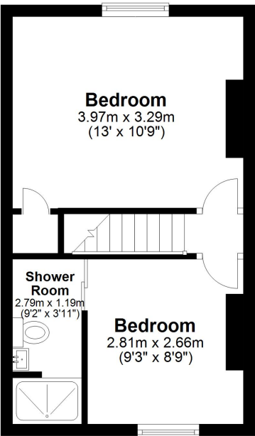
First Floor Approx. 27.4 sq. metres (294.9 sq. feet)
