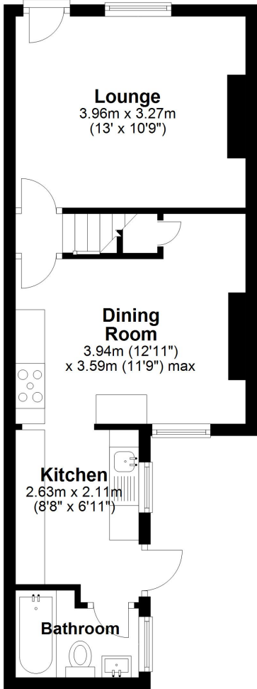
Ground Floor Approx. 39.0 sq. metres (420.2 sq. feet)
