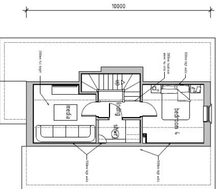
ROOF AREA PLAN
