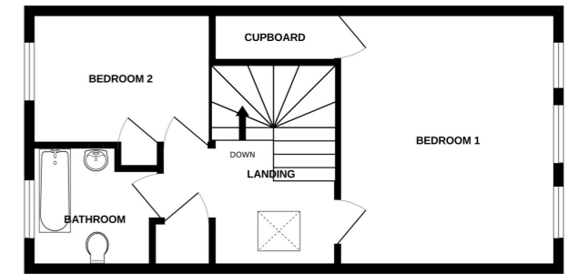
1ST FLOOR 440 sq.ft. (40.9 sq.m.) approx.
