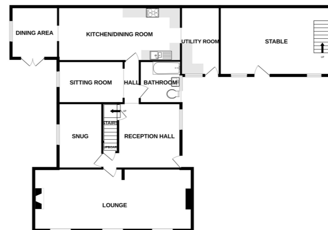
GROUND FLOOR 1549 sq.ft. (143.9 sq.m.) approx.
