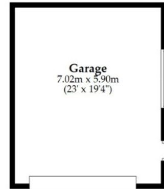
Garage Approx. 41.4 sq. metres (445.8 sq. feet)
