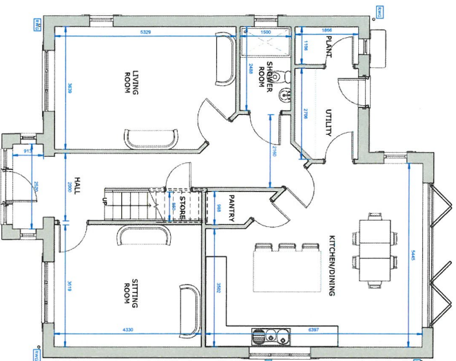
Ground Floor Plan 1:150
