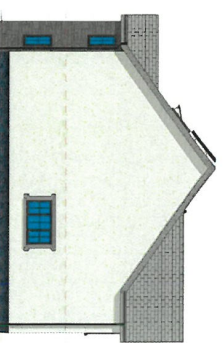
Side 1 Elevation 1:100
