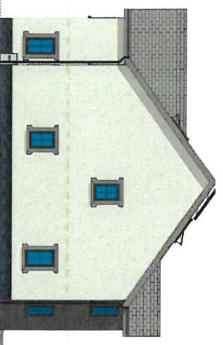
Side 2 Elevation 1:100
