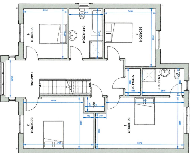
First Floor Plan 1:150
