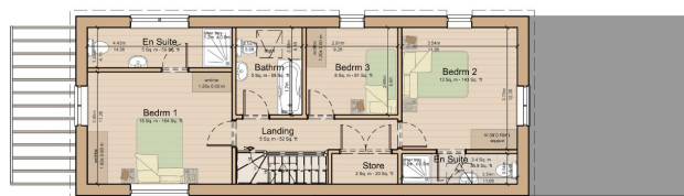
FIRST FLOOR PLAN GIA FLOOR AREA - 63 Sq. m - 681 Sq. ft
