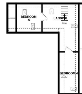
2ND FLOOR
