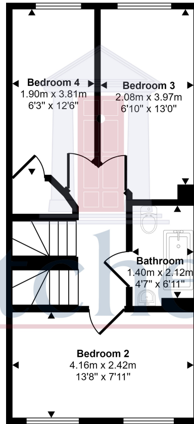
First Floor Approx 39 sq m / 420 sq ft
