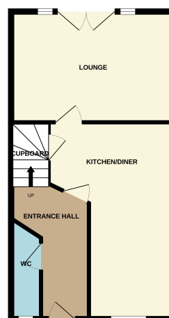
GROUND FLOOR 450 sq.ft. (41.8 sq.m.) approx.
