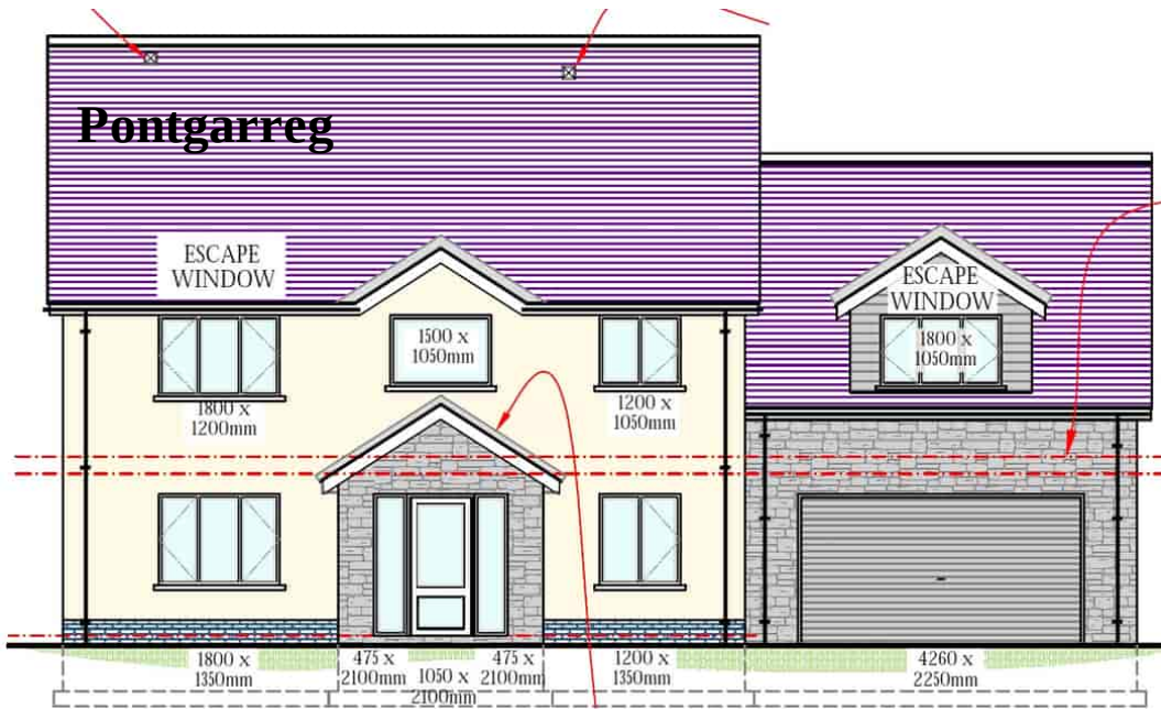
Front Elevation 1:100
