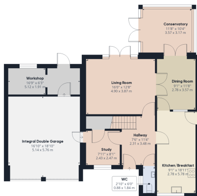
Floor 0
