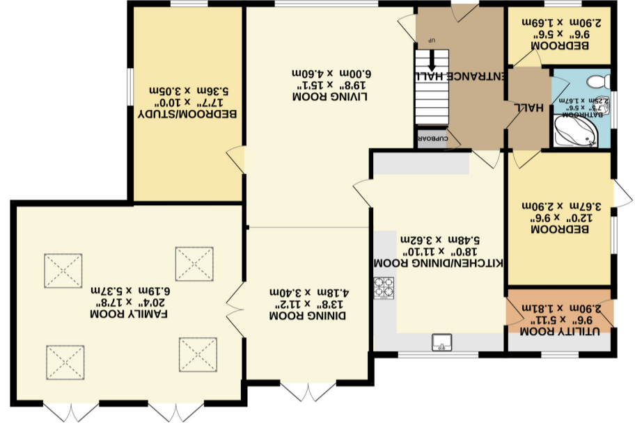
GROUND FLOOR 1567 sq.ft. (145.6 sq.m.) approx.
