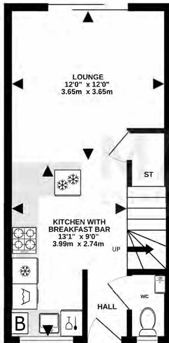
GROUND FLOOR 292 sq.ft. (27.1 sq.m.) approx.
