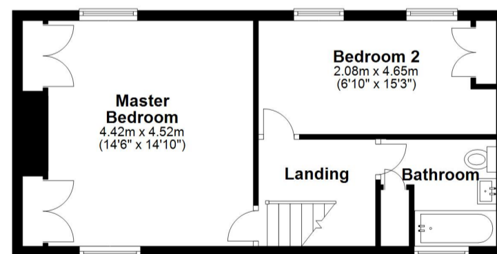
First Floor Approx. 40.3 sq. metres (433.7 sq. feet)
