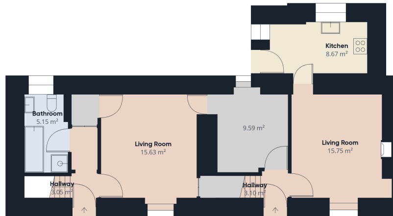
Floor 0
