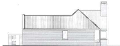
04 | PROPOSED SOUTH ELEVATION Scale 1:100 @ A3
