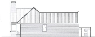
03 | PROPOSED NORTH ELEVATION Scale 1:100 @ A3
