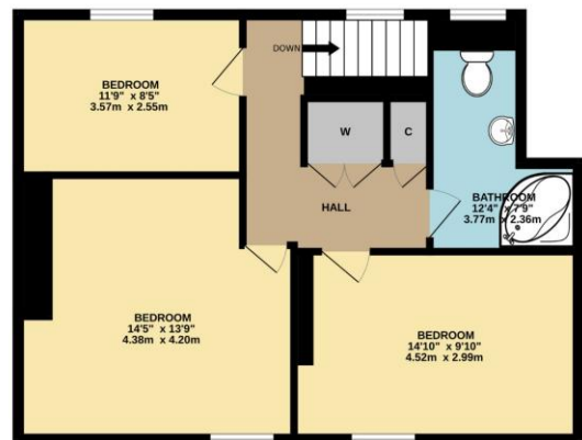
1ST FLOOR 598 sq.ft. (55.5 sq.m.) approx.
