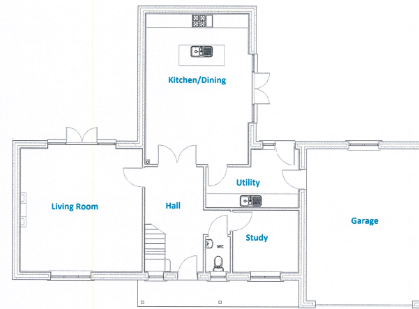
Approx Ground Floor Area = 1286 Sq ft (Including Garage)
