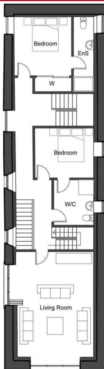
First Floor
