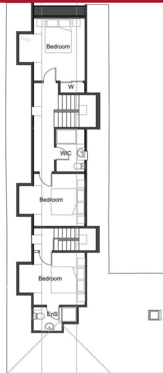
Second Floor
