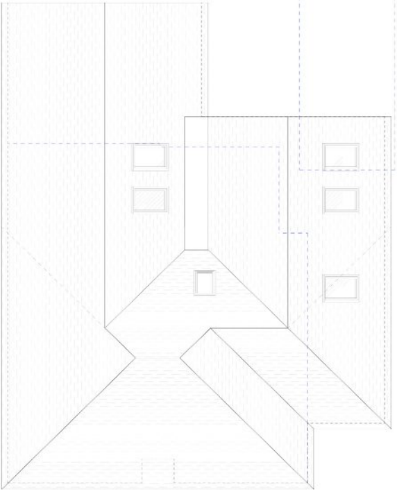
2 proposed roof plan Scale: 1:100
