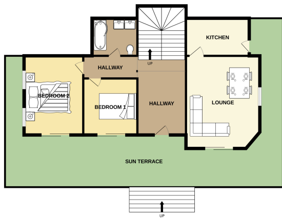
1ST FLOOR 1104 sq.ft. (102.6 sq.m.) approx.
