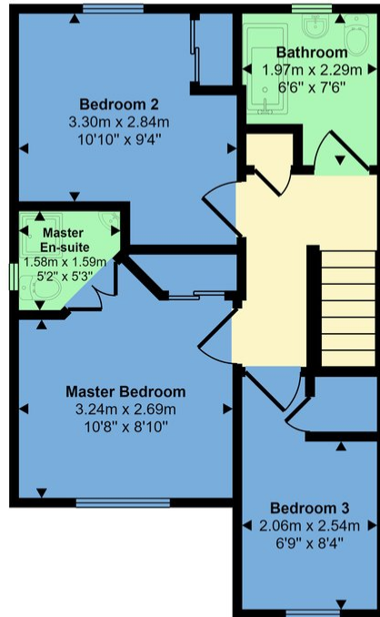
First Floor Approx 43 sq m / 467 sq ft
