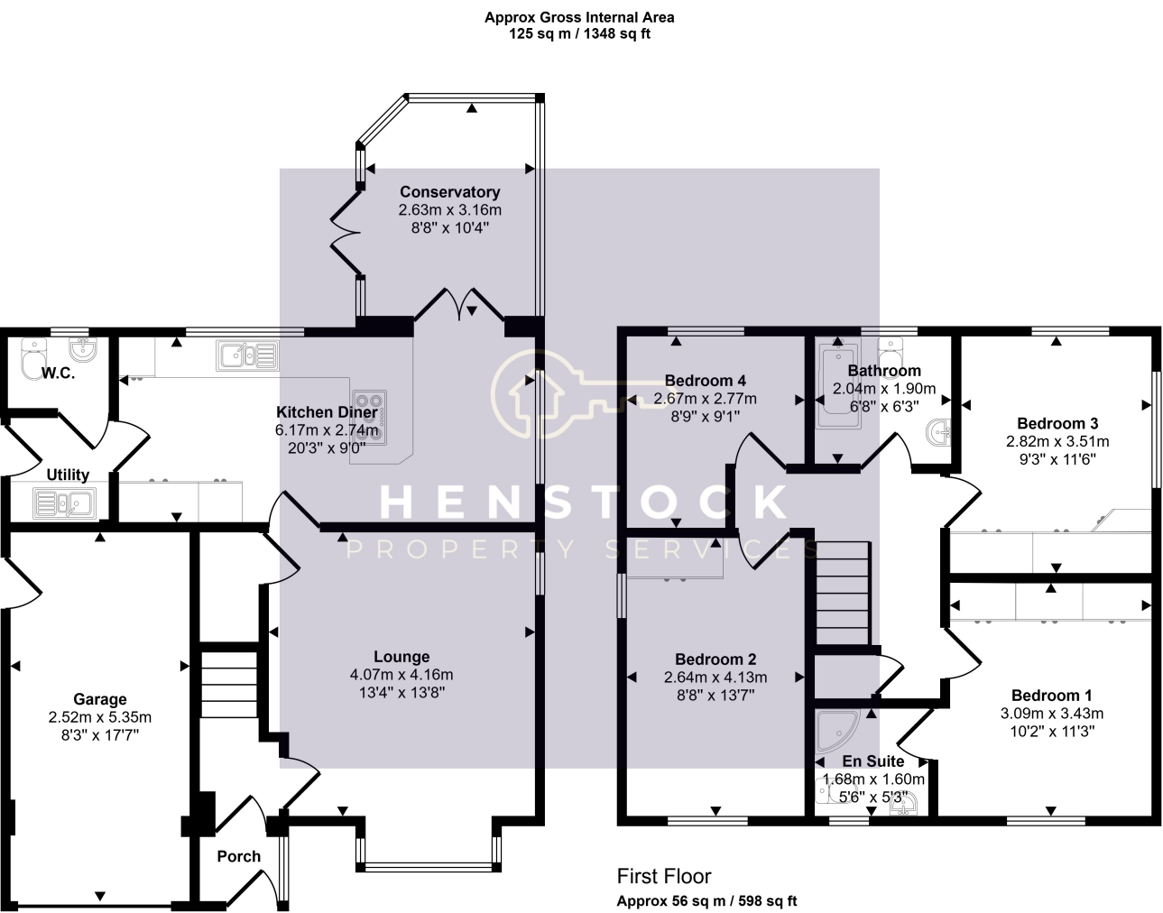
Ground Floor Approx 70 sq m / 750 sq ft
