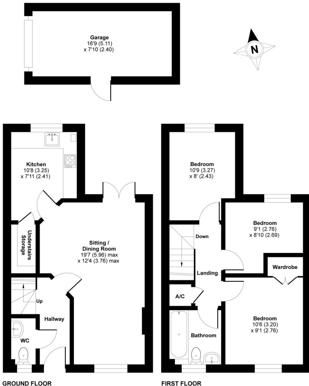
GROUND FLOOR
