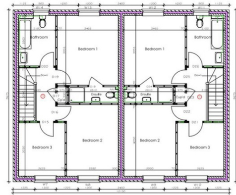
First Floor Plan 1:50
