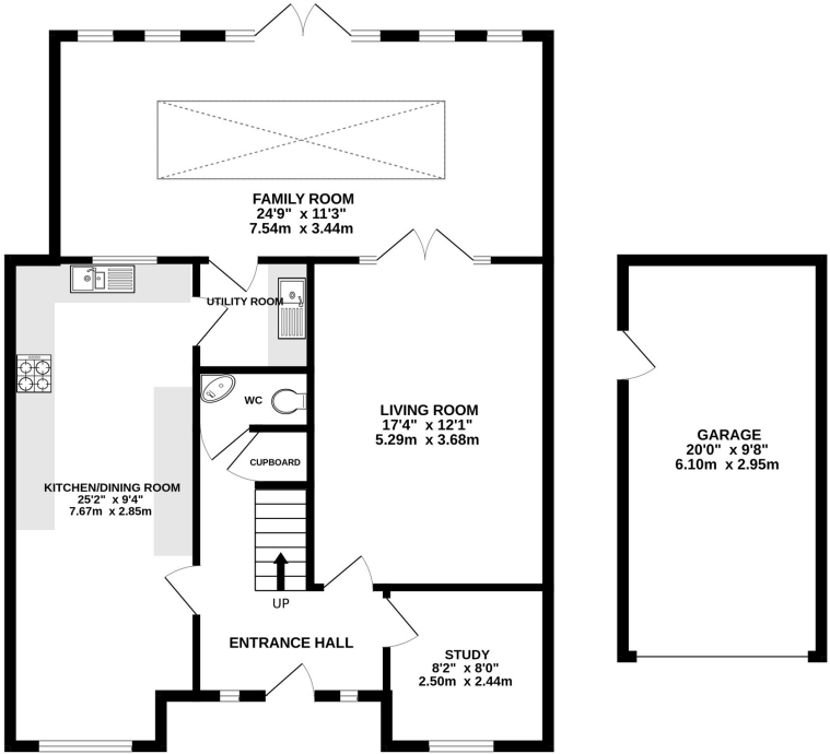
GROUND FLOOR 1141 sq.ft. (106.0 sq.m.) approx.
