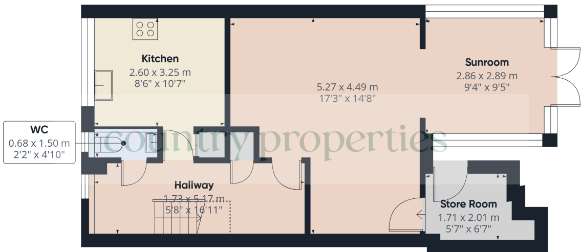
Ground Floor
