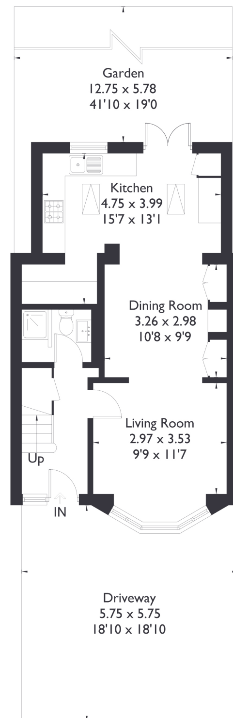
Ground Floor
