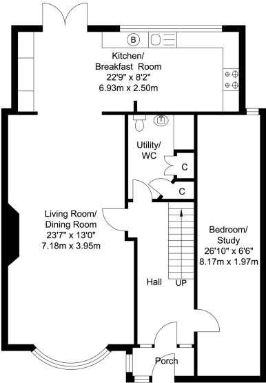
Ground Floor Approximate Floor Area 857.45 SQ.FT. (79.66 SQ.M.)
