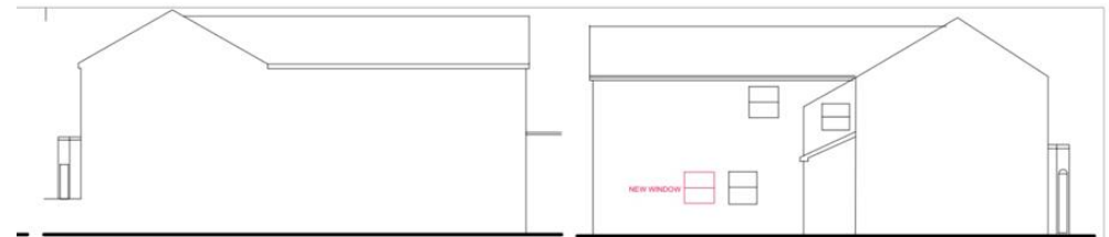
SIDE 1 ELEVATION AS PROPOSED SCALE 1:100
