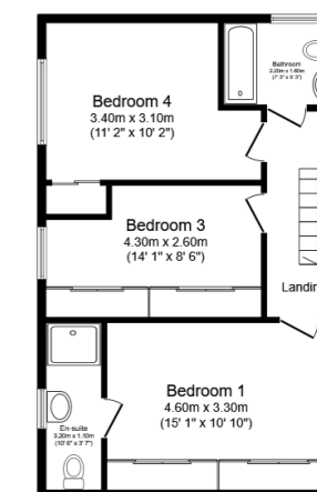
First Floor Floor area 53.0 m 2 (571 sq.ft.)
