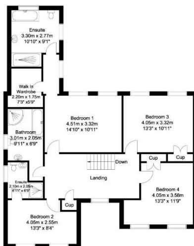
First Floor 95 sq m/1022.57 sq ft Approx.
