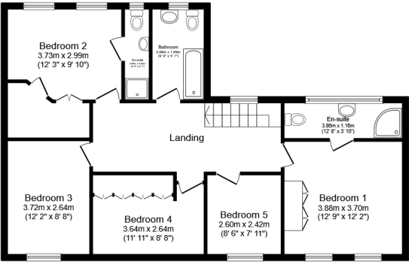
First Floor Floor area 83.9 m² (903 sq.ft.)
