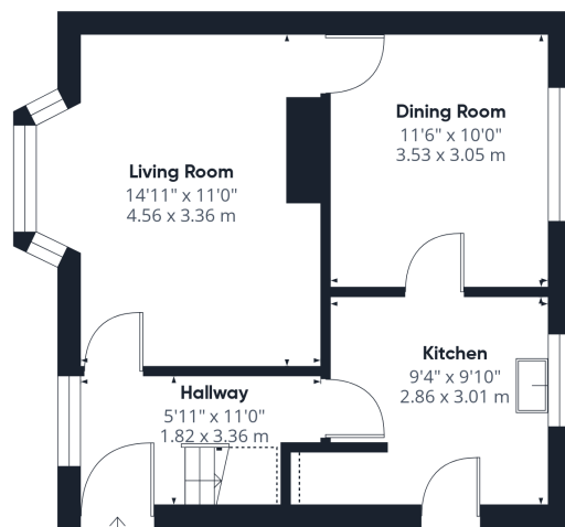
Floor 0 Building 1
