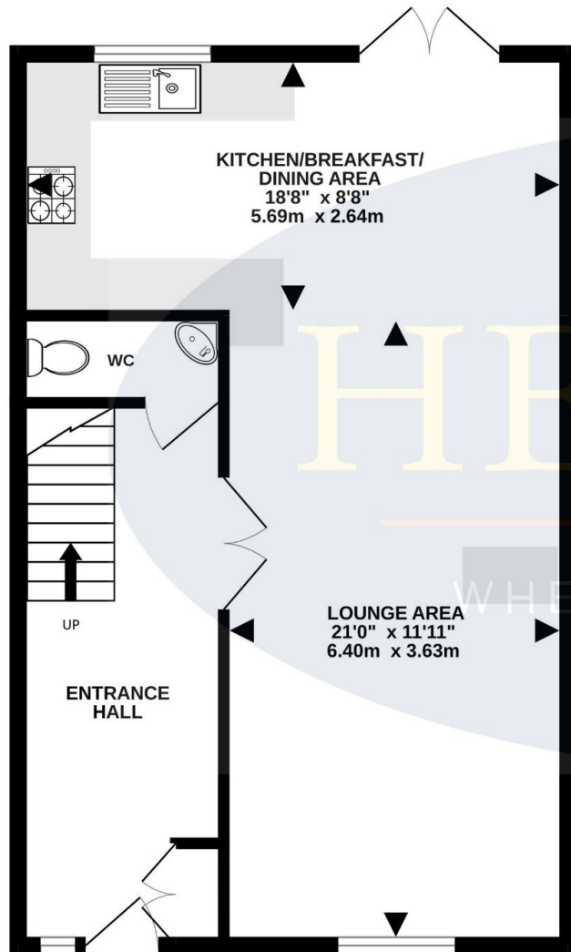
GROUND FLOOR 561 sq.ft. (52.2 sq.m.) approx.
