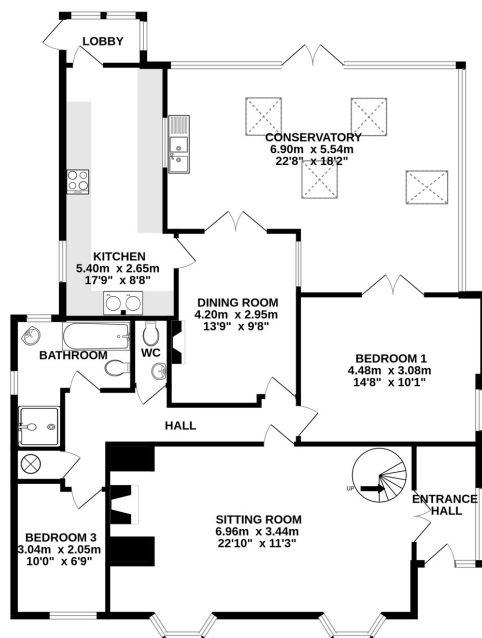
GROUND FLOOR 139.2 sq.m. (1499 sq.ft.) approx.
