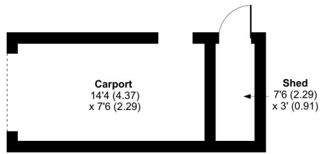
OUTBUILDING
