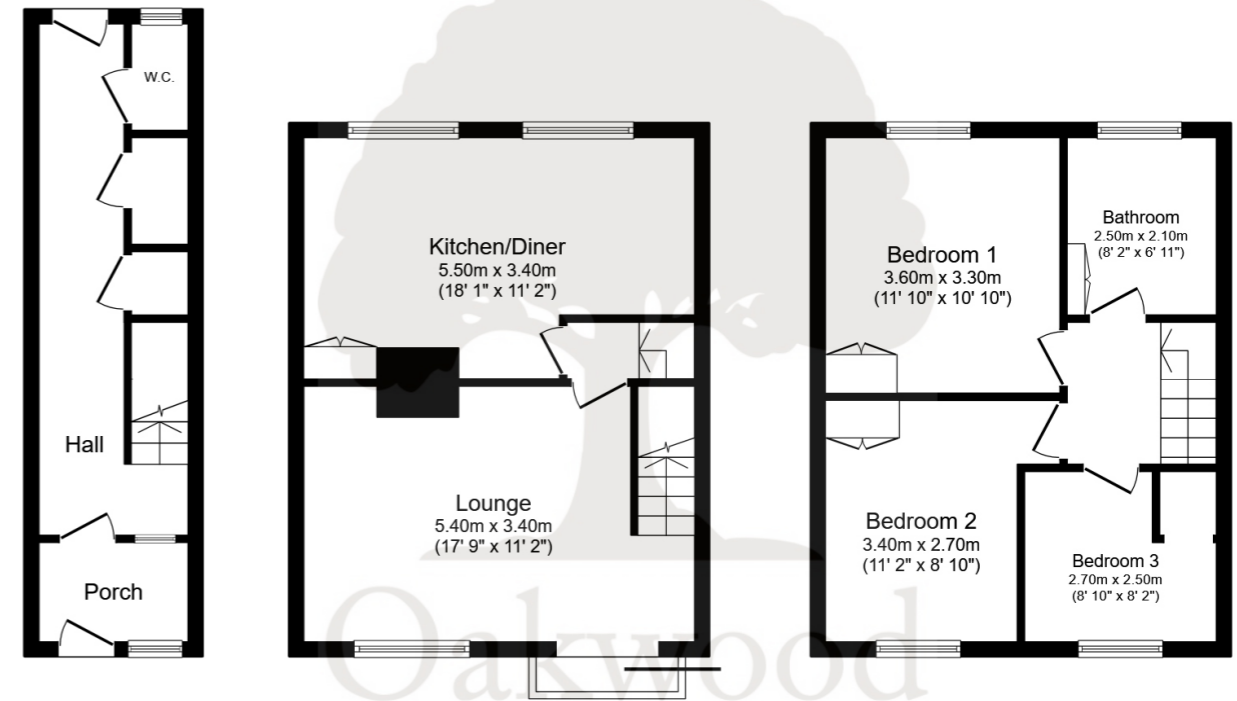
Ground Floor Floor area 18.3 sq.m. (197 sq.ft.) First Floor Floor area 39.1 sq.m. (420 sq.ft.) Second Floor Floor area 39.0 sq.m. (420 sq.ft.)
