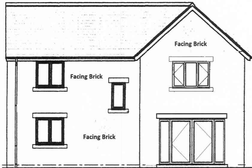
WEST ELEVATION
