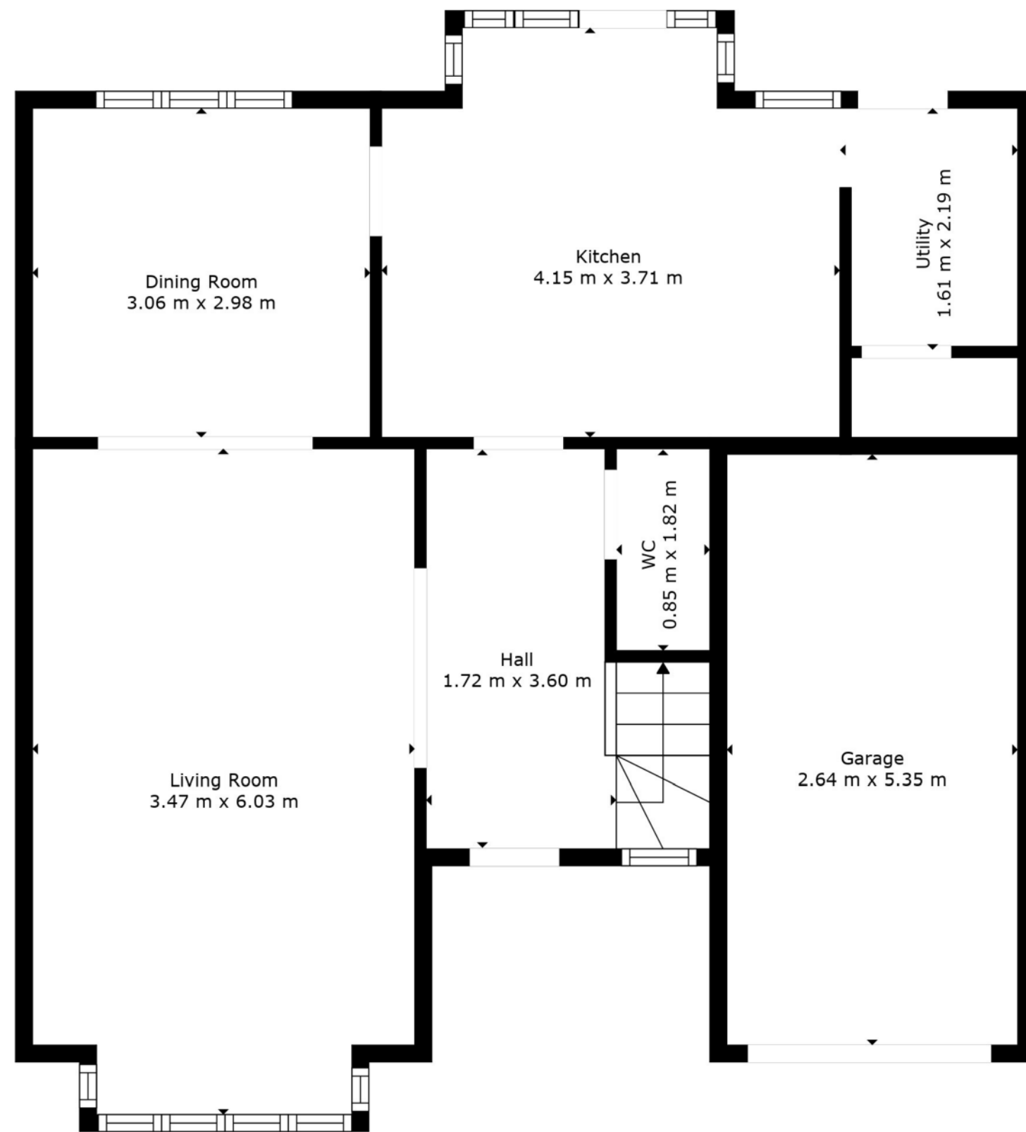
Floor 1
