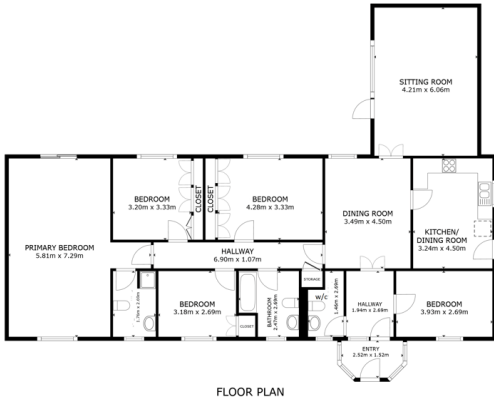
FLOOR PLAN
