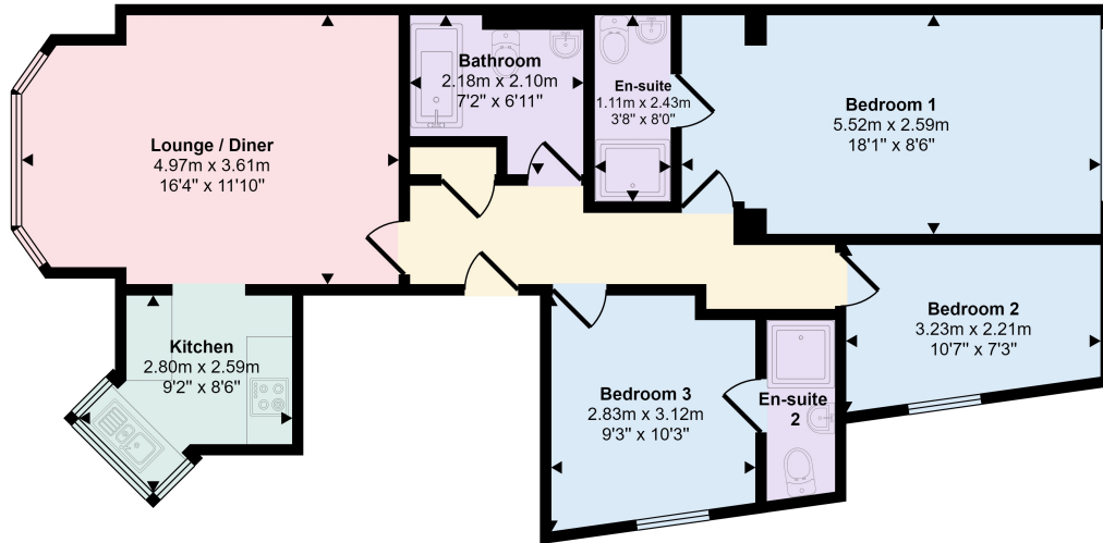
Floorplan
