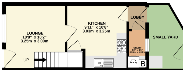
GROUND FLOOR 246 sq.ft. (22.9 sq.m.) approx.
