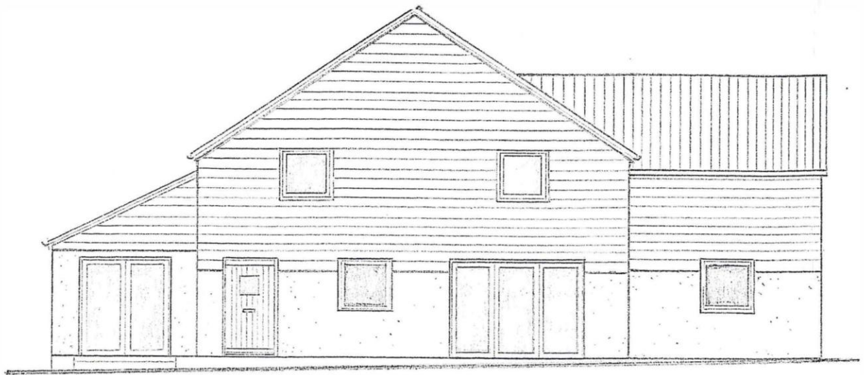
South Elevation
